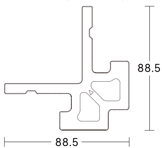
OUTER CORNER (VERTICAL)-HLYC-021F
