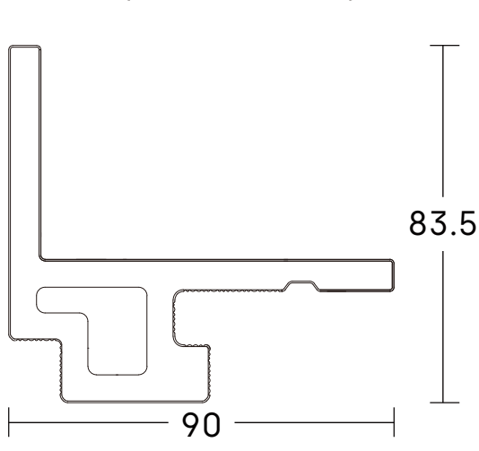
F-TRIM(HORIZONTAL)-HLYC-019F
