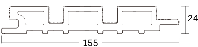
CASTELLATED CLADDING BOARD-HLYC-018F
